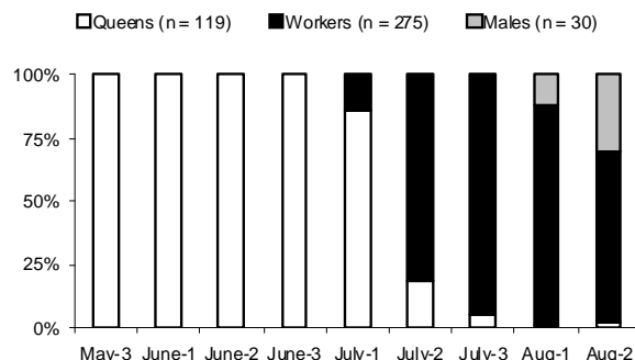
Fig. 1. The caste composition of B. distinguendus seen foraging on bee walks on South Uist during each time period in 2005.
